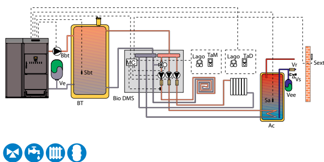
MODUL BIO DMS + BT
