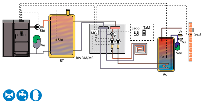
MODUL BIO DM/MS + BT
